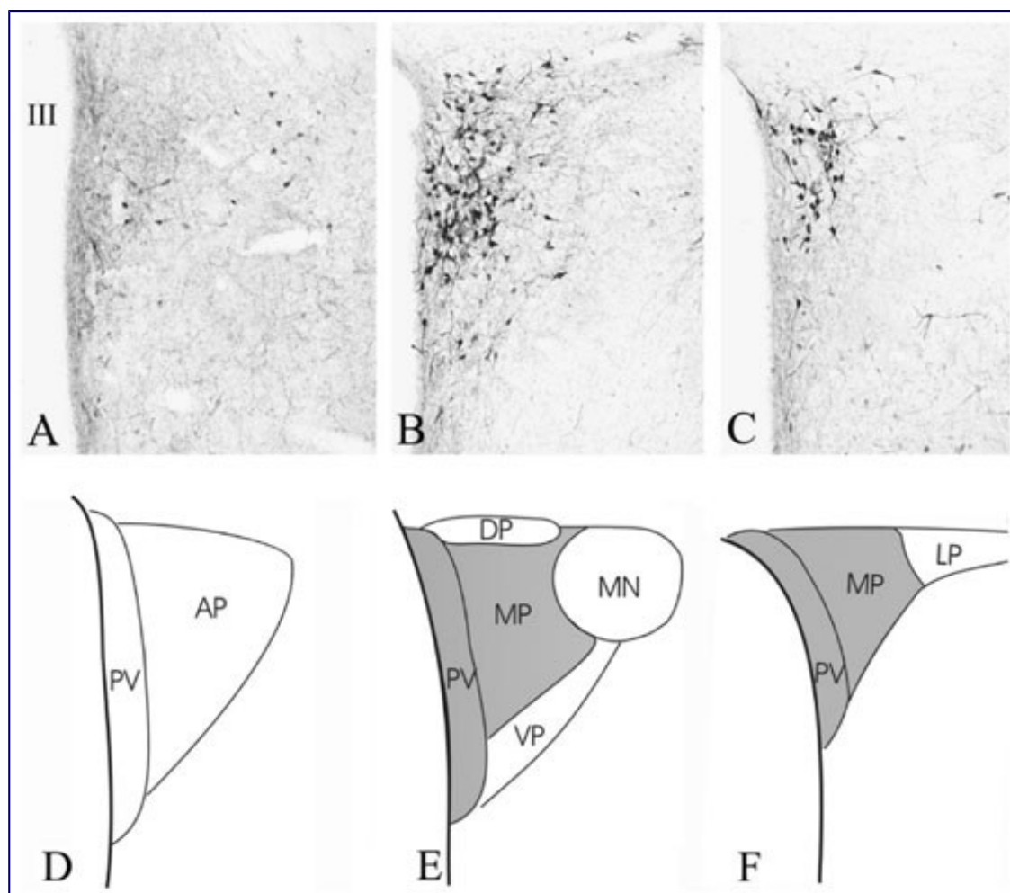
Figure 4.9 (new) Distribution of TRH-synthesizing neurons in the PVN. Low power micrographs (A–C) illustrate the TRH neurons at three rostrocaudal levels of the PVN. Schematic drawings (D–F) illustrate the subdivisions of the PVN where hypophysiotropic TRH neurons are localized (gray). AP, anterior parvocellular subdivision; DP, dorsal parvocellular subdivision; LP, lateral parvocellular subdivision; MN, magnocellular part of PVN; MP, medial parvocellular subdivision, PV,
