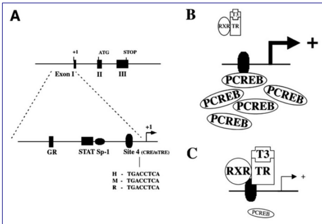
Figure 4-10 (new) Genomic and promoter structure of TRH. The murine, rat and human TRH genes are composed of three exons and two introns (A). The coding sequence for the precursor protein is present on exons 2 and 3. As depicted, the TRH promoter region precedes the transcription start site in exon 1. The proximal 250-bp sequences of the human, mouse and rat promoters are similar and share the indicated transcription factor binding sites. The location of the CREB binding site (Site 4) and sequences in human (H), mouse (M) and rat (R) are shown. (B,C) Hypothesized schematic representation of the interaction between PCREB and the thyroid hormone receptor at Site 4. (B) Illustrates that in the presence of abundant PCREB, there may be less availability for binding of the thyroid hormone receptor/T3 complex, hence, an increase in TRH gene transcription. When PCREB concentrations fall as shown in (C), increased binding of the thyroid hormone receptor/T3 complex reduces TRH gene transcription (From (112) with permission)
