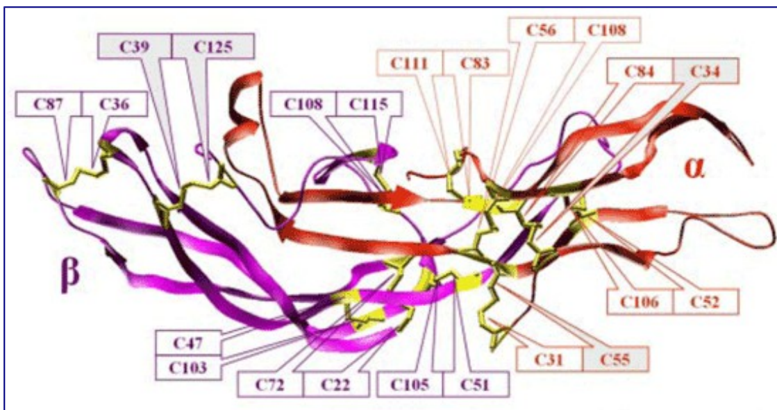
Figure 4-3 (new) Structural model of TSH based on the FSH x-ray structure, which is the best available structural template for TSH. The boxed residue numbers represent cysteines residues, which form stabilizing disulfide bridges (yellow): 5 in alpha-subunit (red orange), and 6 in the beta-subunit (magenta). The disulfide bridge (C39/C125) toward the C-terminal tail of the beta-subunit of TSH that wraps around the beta-subunit like a “seat belt” stabilizes the heterodimerization of TSH as well and also in FSH, LH, and CG. (Reproduced from Kleinau et al.(16), with permission)
