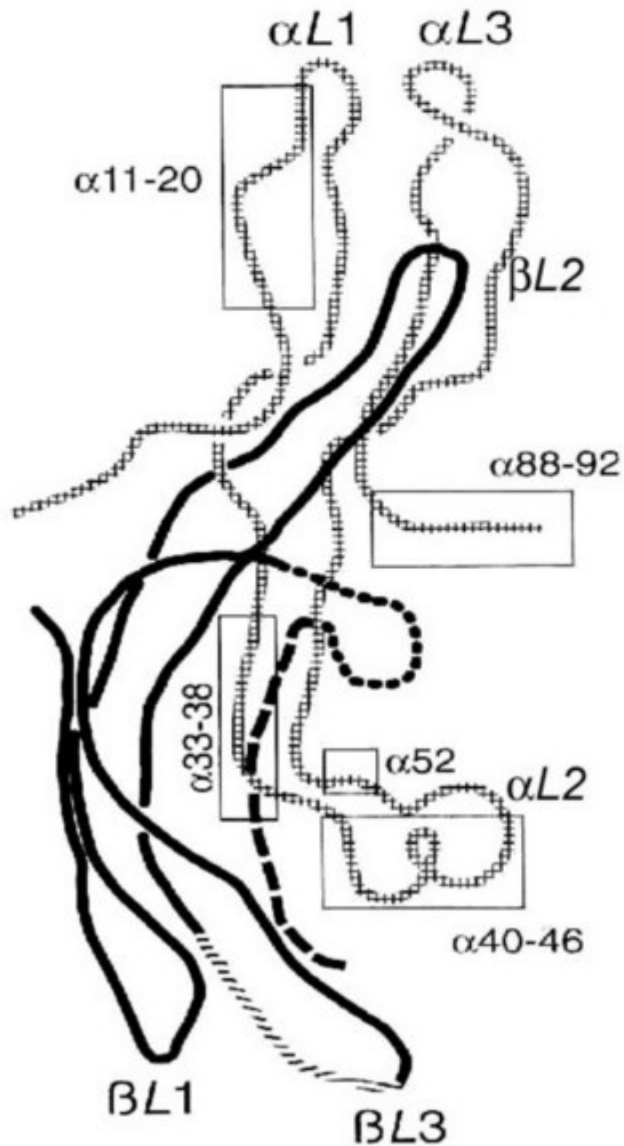
Figure 4-2 Schematic drawing of human TSH, based on a molecular homology model built on the template of a hCG model 14 . The \alpha -subunit is shown as checkered, and the \beta -subunit as a solid line. The two hairpin loops in each subunit are marked L1, L3; each subunit has also a long loop (L2), which extends from the opposite site of the central cystine knot. The functionally important \alpha -subunit domains are boxed. Important domains of the \beta -subunit are marked directly within the line drawing (crossed line, beaded line and dashed line): For further details the reader is referred to Grossman et al. 2 . (Reproduced from Grossman et al. (2) , with permission).
