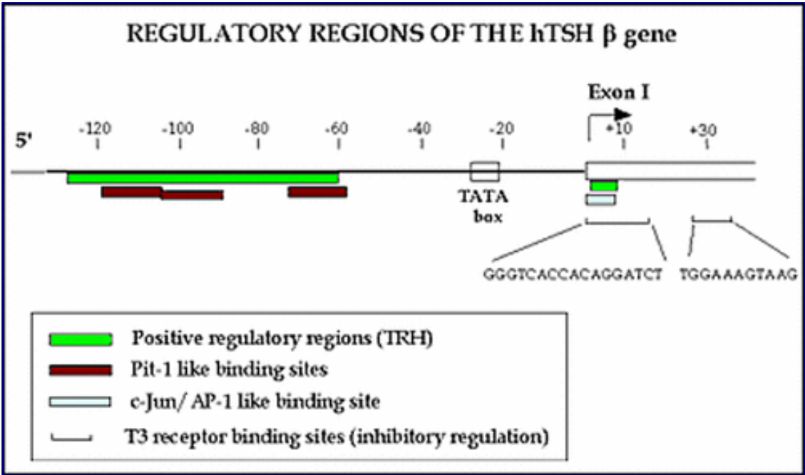
Figure 4- 13 The regulatory region of human TSH- \beta gene (see text for details)
