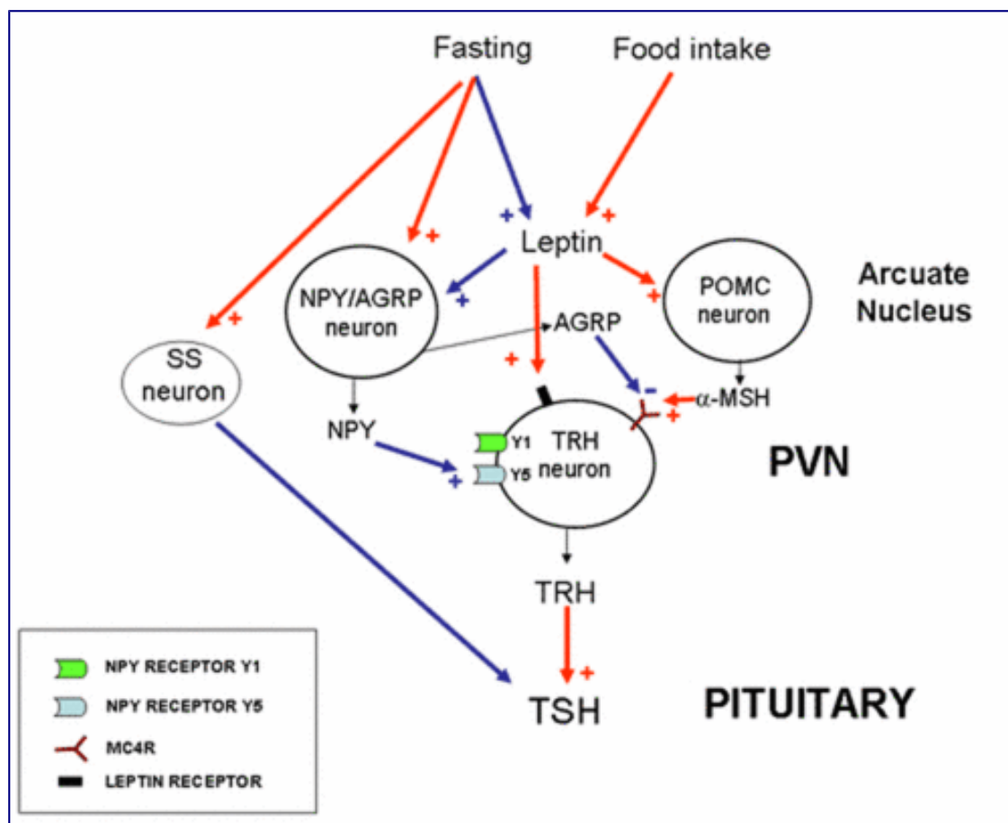
Figure 4- 15 Role fasting, somatostatin (SS) pathways and leptin on TRH and TSH secretion. POMC: pro-opiomelanocortin; α-MSH: α-melanocyte-stimulating hormone; AGRP: Agouti receptor protein; NPY: neuropeptide Y; MC4R: melanocortin 4 receptor; PVN: paraventricular nucleus Red arrows: stimulation; blue arrows: inhibition; for further details, see text.
